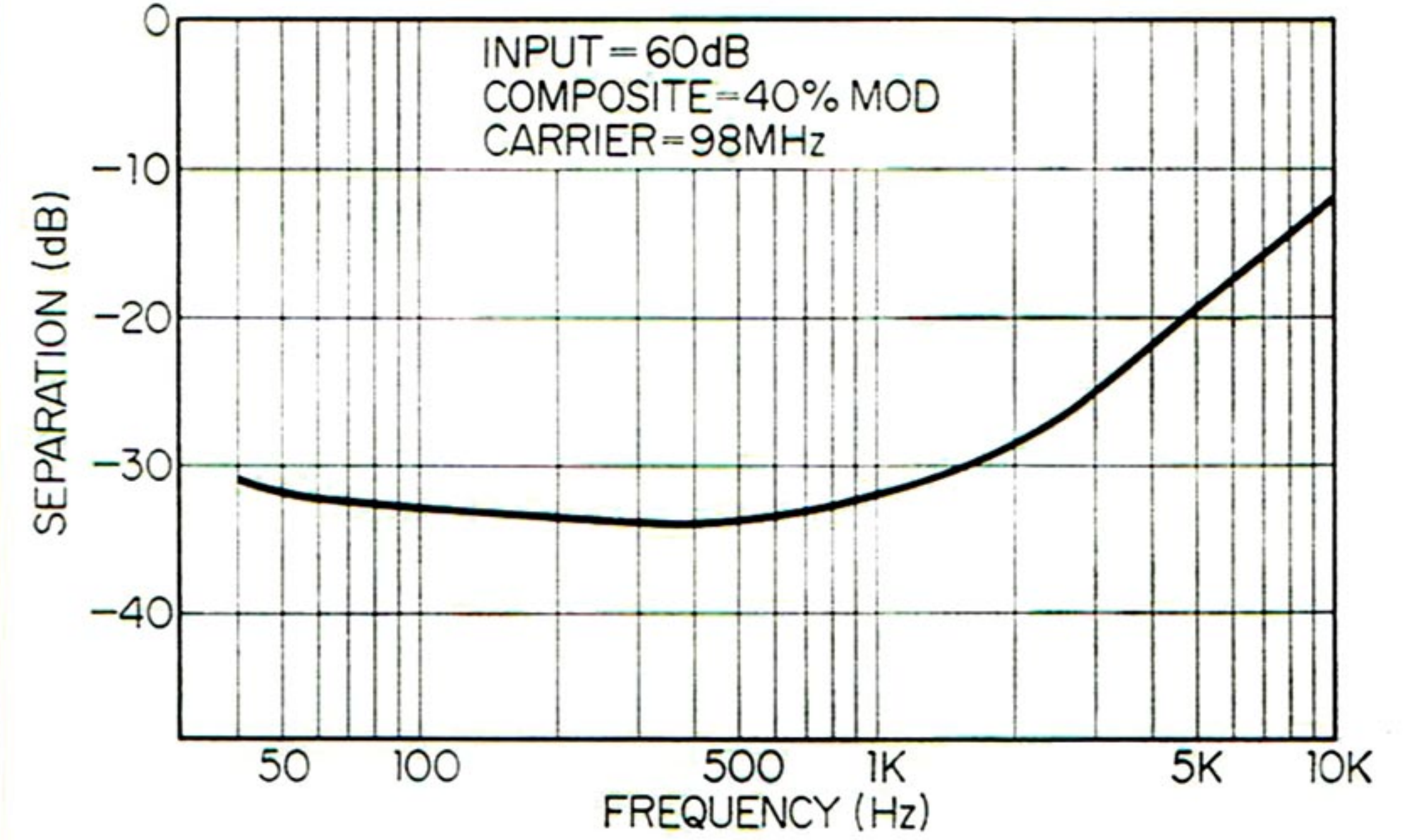
FM STEREO SEPARATION
