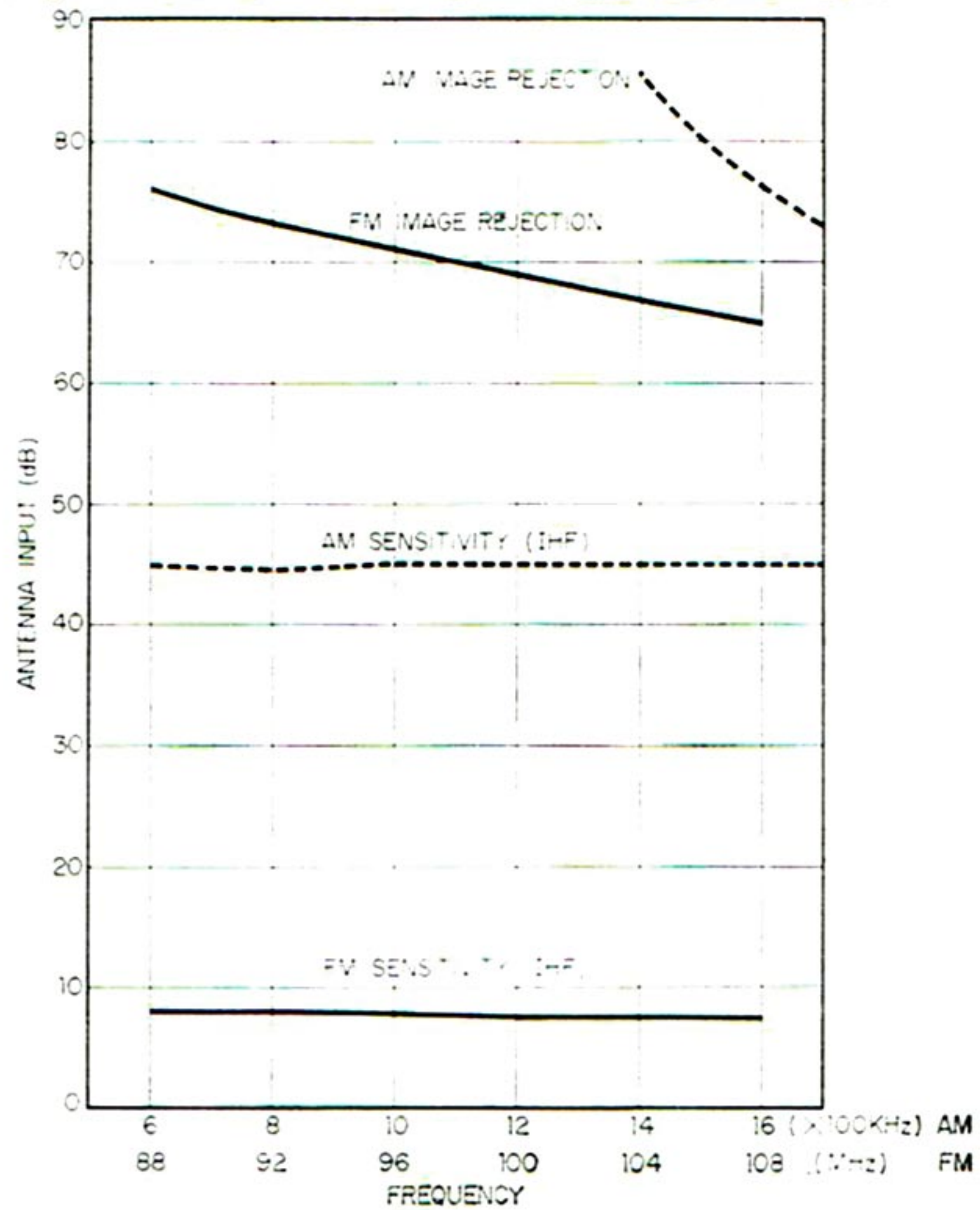
FM, AM SENSITIVITY & IMAGE REJECTION
