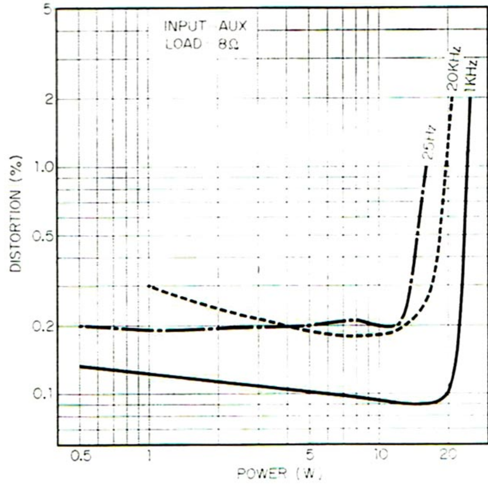
POWER OUTPUT HARMONIC DISTORTION
