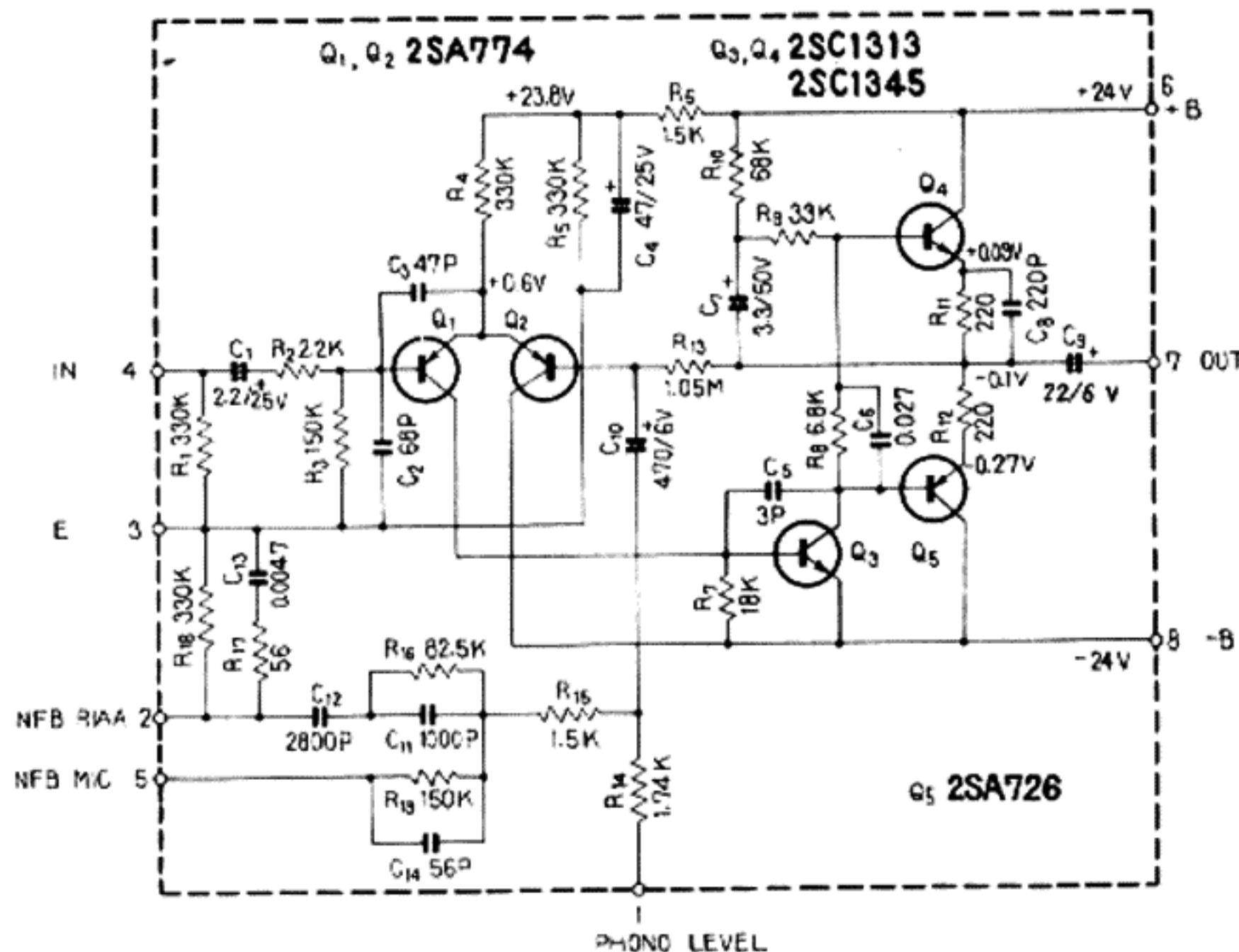
EQUALIZER AMP, CIRCUIT SCHEMATIC
