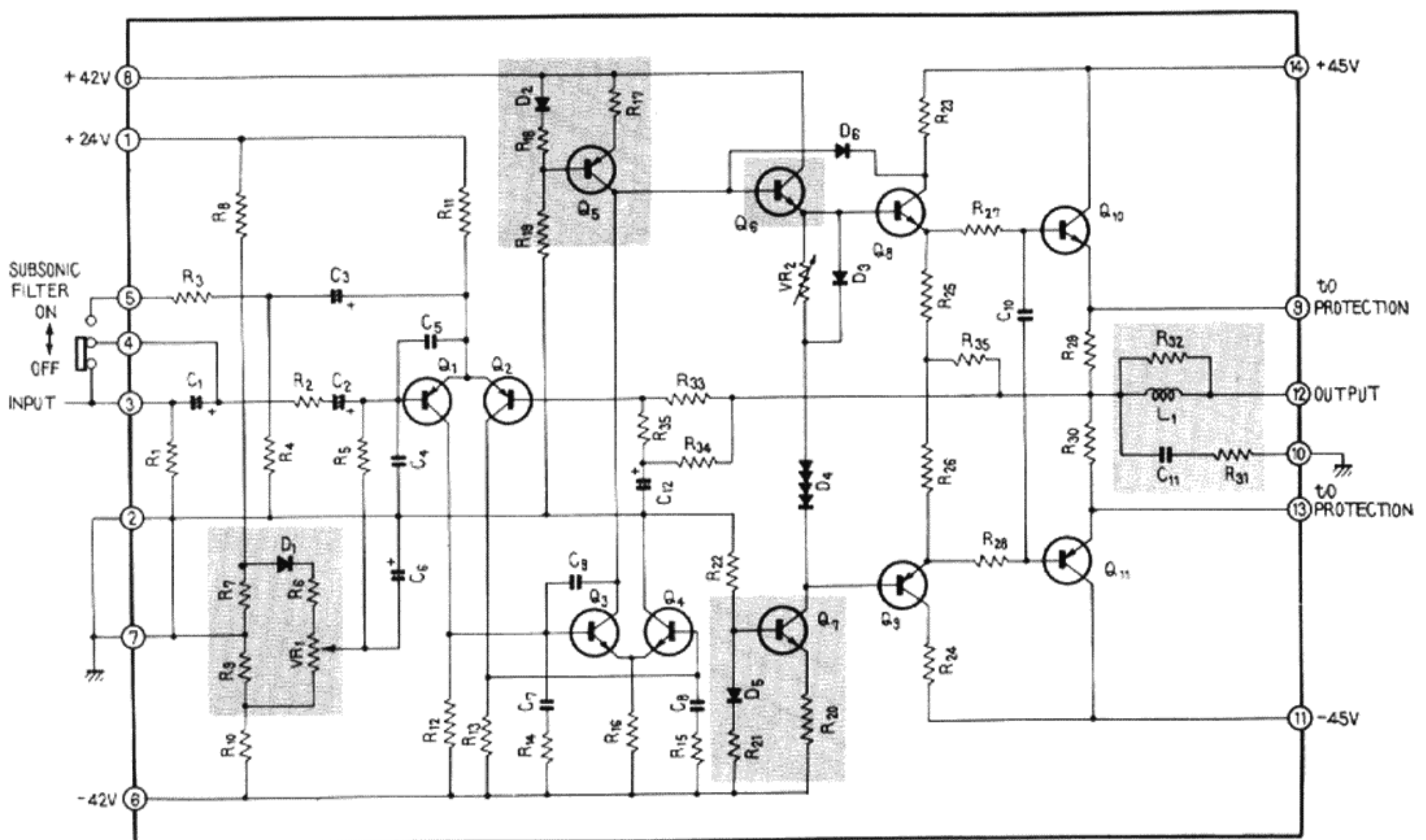
POWER AMP, CIRCUIT SCHEMATIC
